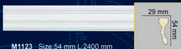
M1123 Size:54 mm L:2400 mm
