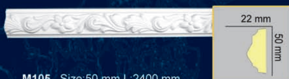
M105 Size:50 mm L:2400 mm
