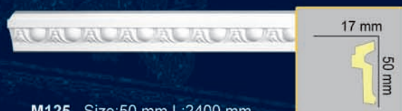
M125 Size:50 mm L:2400 mm
