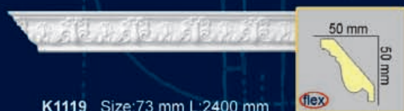
K1119 Size: 73 mm L: 2400 mm
