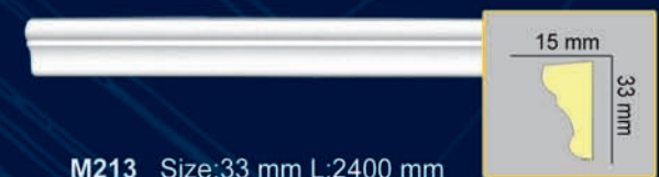
M213 Size:33 mm L:2400 mm
